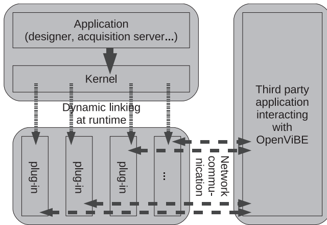
Figure 7. Software architecture.
